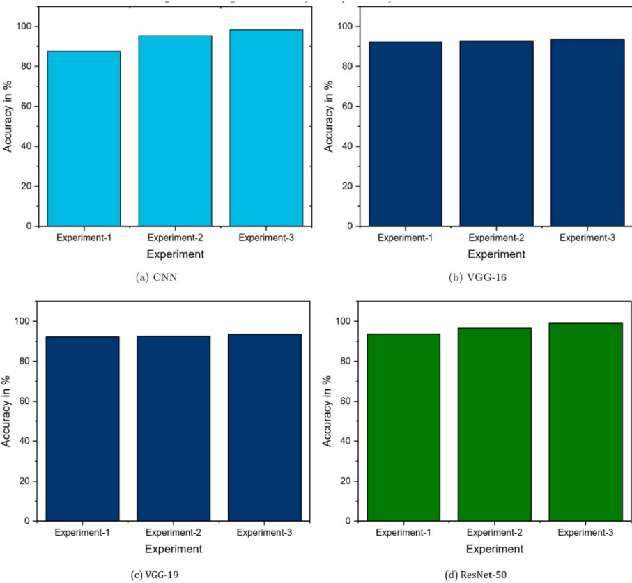
Fig. 5. Accuracy results.
